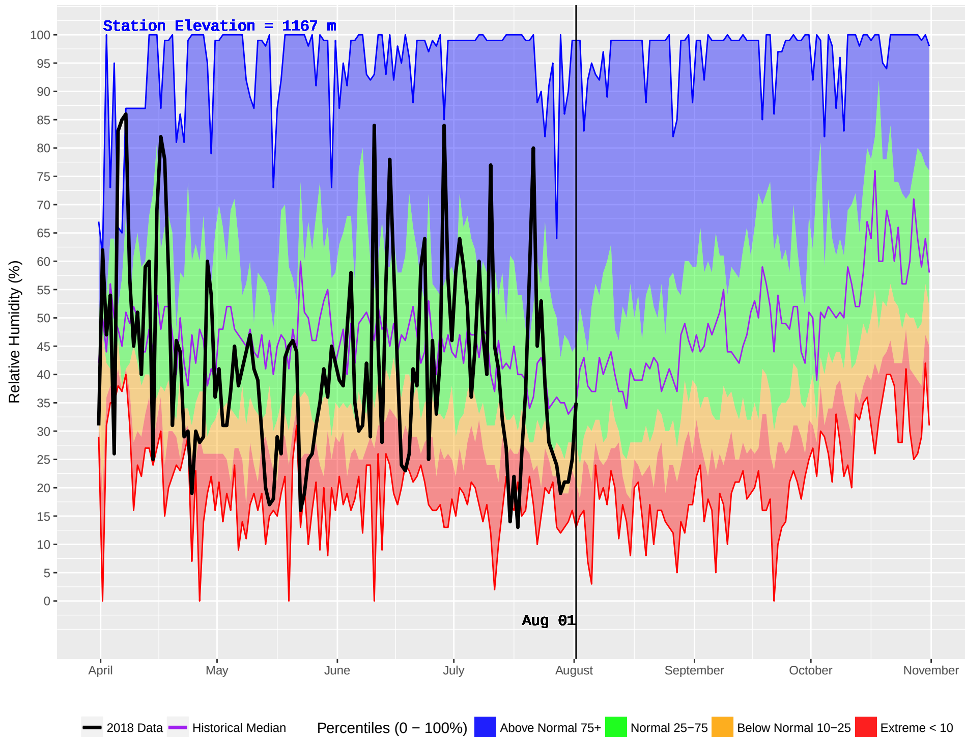
LEIGHTON LAKE (307) : Historical (1982–2016) and Current (2018) Daily Relative Humidity
