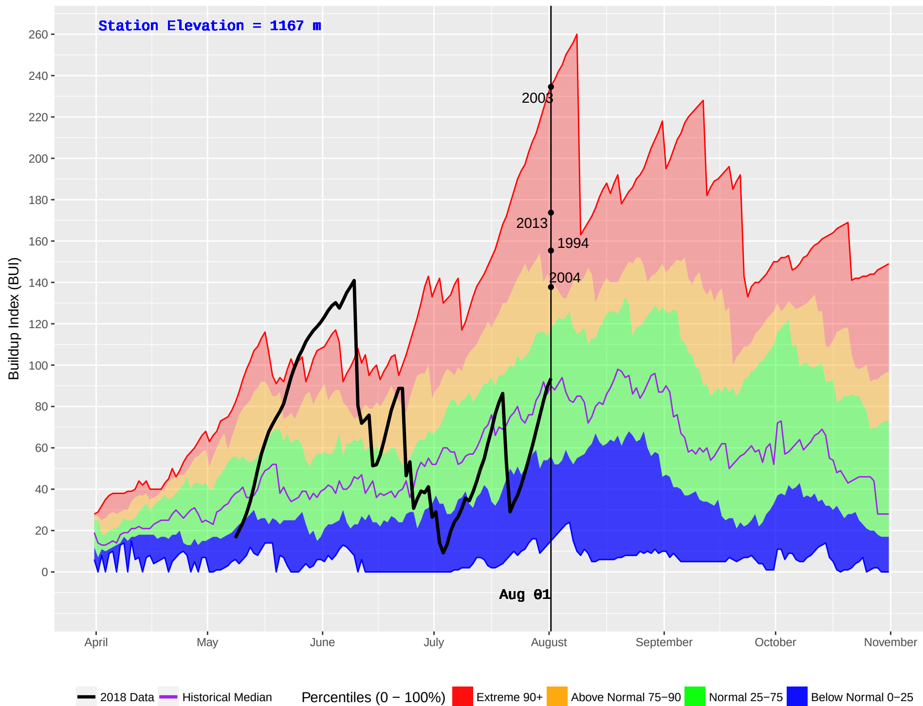
LEIGHTON LAKE (307) : Historical (1982–2016) and Current (2018) Daily Buildup Index (BUI)
